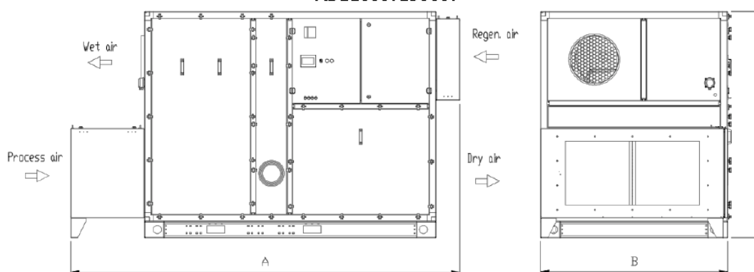
AD11000÷15000T
