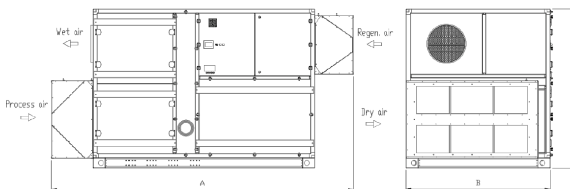
AD19000÷25000
